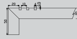
20-ME50-3GM 20mm Mitred Edge Stair Tread with 50mm Dropdown and 3 Anti-slip Metal Inserts
