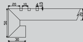
20-GRAD50-3GM 20mm Mitred Gradone Stair Tread with 50mm Dropdown and 3 Anti-slip Metal Inserts
