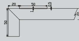
20-ME50-50GR 20mm Mitred Edge Stair Tread with 50mm Dropdown and 50mm Anti-slip Resin Strip
