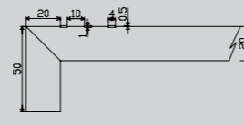
20-ME50-3GR 20mm Mitred Edge Stair Tread with 50mm Dropdown and 3 Anti-slip Resin Inserts
