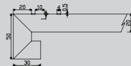
20-GRAD50-3GR 20mm Mitred Gradone Stair Tread with 50mm Dropdown and 3 Anti-slip Resin Inserts
