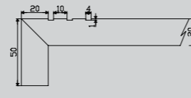
20-ME50-3G 20mm Mitred Edge Stair Tread with 50mm Dropdown and 3 Anti-slip Grooves
