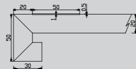
20-GRAD50-50GR 20mm Mitred Gradone Stair Tread with 50mm Dropdown and 50mm Anti-slip Resin Strip
