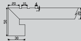
20-GRAD50-3G 20mm Mitred Gradone Stair Tread with 50mm Dropdown and 3 Anti-slip Grooves
